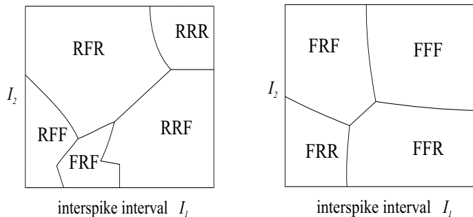
Figure 3: (A, left) Most likely release pattern of a synapse in dependence of the interspike intervals I_1 and I_2 . The synaptic parameters are C_0 = 1.5 , V_0 = 0.5 , \tau_C = 5 , \tau_V = 9 , \alpha = 0.7 . (B, right) Release patterns for a synapse with other values of its parameters ( C_0 = 0.1 , V_0 = 1.8 , \tau_C = 15 , \tau_V = 30 , \alpha = 1 ).
