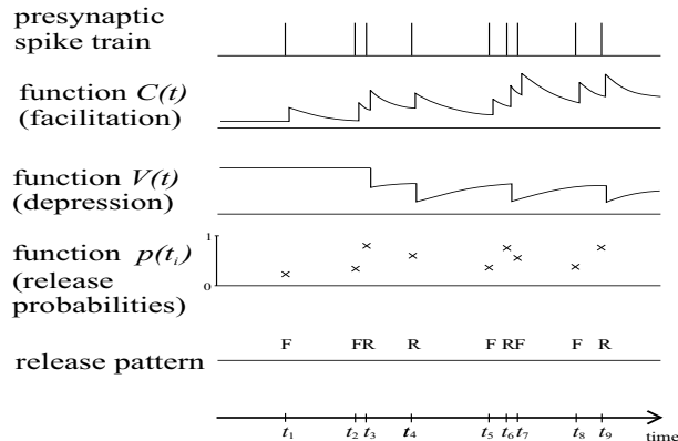
Figure 1: Synaptic computation on a spike train \underline{t} , together with the temporal dynamics of the internal variables C and V of our model. Note that V(t) changes its value only when a presynaptic spike causes release.
