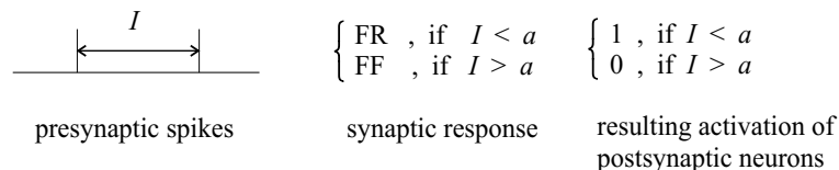
Figure 5: A mechanism for translating temporal coding into population coding.
