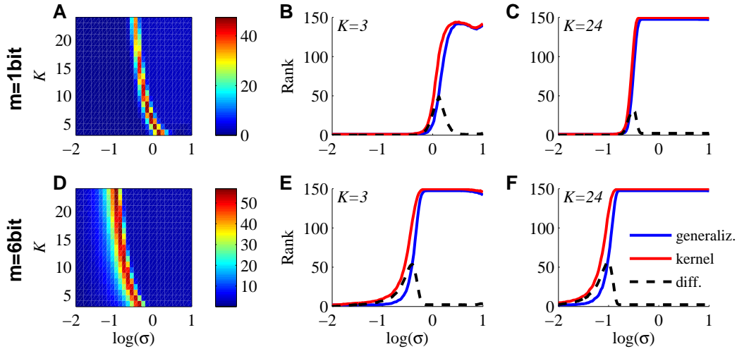
Figure 3: Kernel-quality and generalization rank of quantized ESNs of size N = 150 . Upper plots are for binary reservoirs ( m = 1 bit), lower plots for high resolution reservoirs ( m = 6 bit). A ) The difference between the kernel-quality and the generalization rank as a function of the log STD of weights and the in-degree K . B ) The kernel-quality (red), the generalization rank (blue) and the difference between both (black) for K = 3 as a function of \log(\sigma) . C ) Same as panel B, but for an in-degree of K = 24 . In comparison to panel B, the transition of both measures is much steeper. D,E,F ) Same as panels A, B, and C respectively, but for a high resolution reservoir. All plotted values are means over 100 independent runs with randomly drawn networks, initial states, and input streams.
