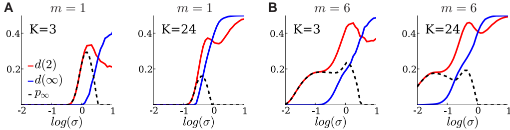
Figure 5: Contributions d(2) and d(\infty) to the mean-field predictor p_\infty for different quantization levels m \in \{1, 6\} and different in-degrees K \in \{3, 24\} as a function of STD \sigma of the weights. The plots show slices of the 2d plots Fig. 4A and C for constant K . A ) For m = 1 it can be seen that the region in \log(\sigma) -space with high d(2) and low d(\infty) is significantly larger for K = 3 than for K = 24 . B ) For m = 6 this region is roughly independent of K except a shift.
