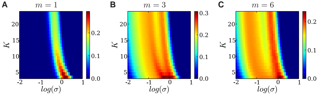
Figure 4: Mean-field predictor p_\infty for computational power for different quantization levels m as a function of the STD \sigma of the weights and in-degree K . A) m = 1 . B) m = 3 . C) m = 6 . Compare this result to the numerically determined performance p_{\text{exp}} plotted in Fig. 1.
